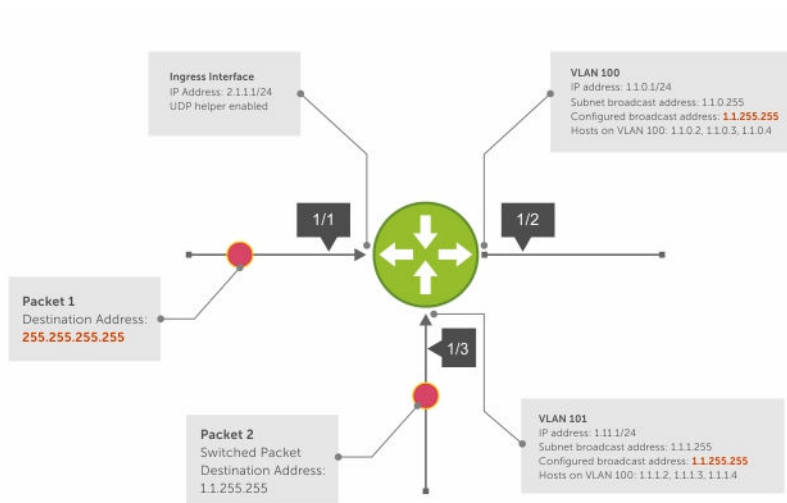
Figure 46. UDP Helper with Configured Broadcast Addresses
